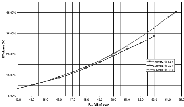
Efficiency of P150-UHF-H @ 32V
