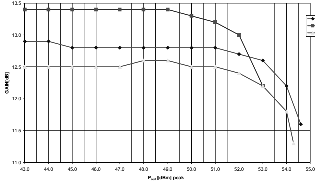
Power Gain of P150-UHF-H @ 32V
