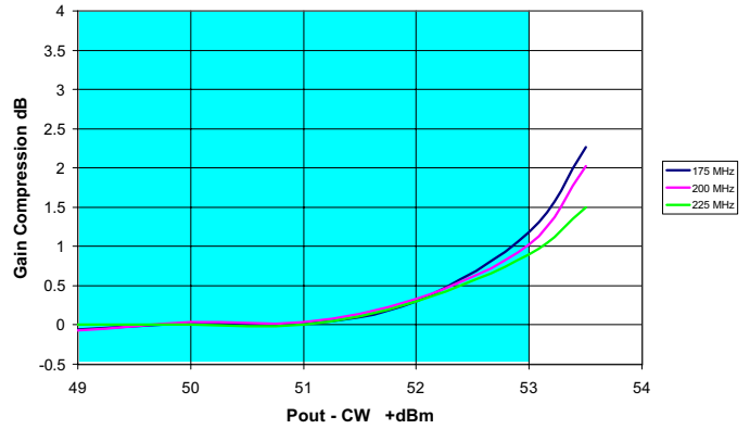
Gain Compression
