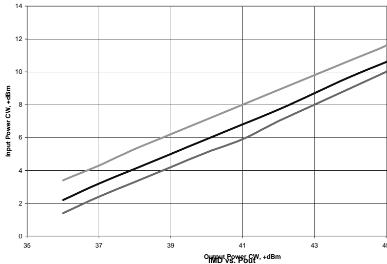
Pin Vs. Pout
