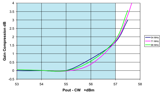
Gain Compression
